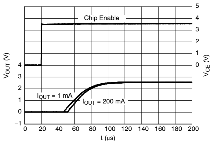
Figure 41. Start-up, 2.5 V Version, V_{\text{IN}} = 3.5 \text{ V}
