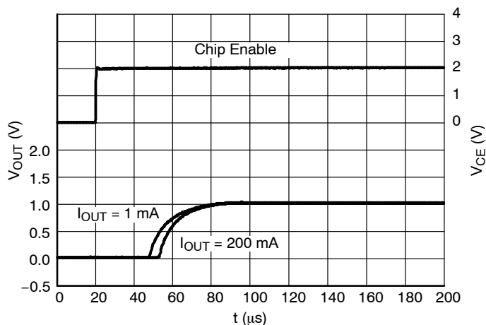
Figure 39. Start-up, 1.0 V Version, V_{\text{IN}} = 2.0 \text{ V}
