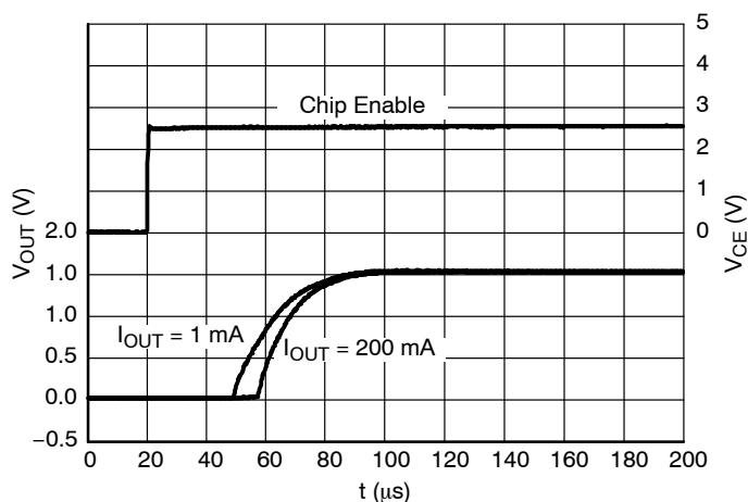
Figure 40. Start-up, 1.5 V Version, V_{\text{IN}} = 2.5 \text{ V}
